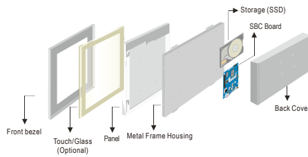
Modularized Construction
