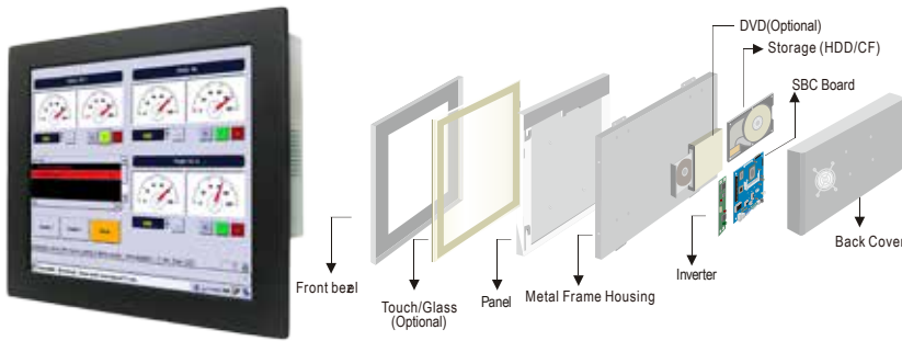
Mechanical design
