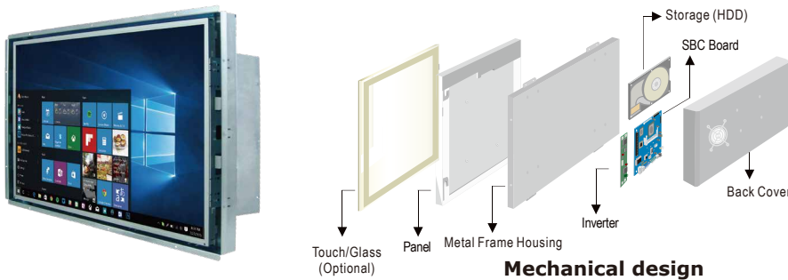
Open Frame
