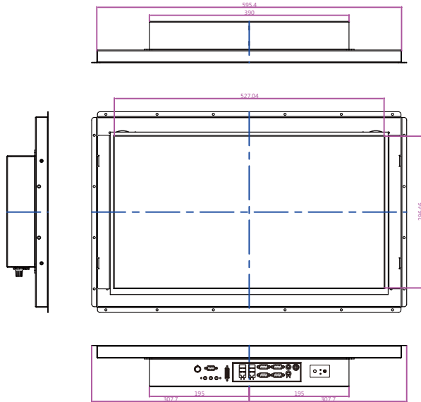
Open Frame
