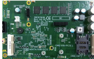
2 x PCI Express Mini Card slot + 1 x SIM Card slot Excellent extensibility in such compact size
